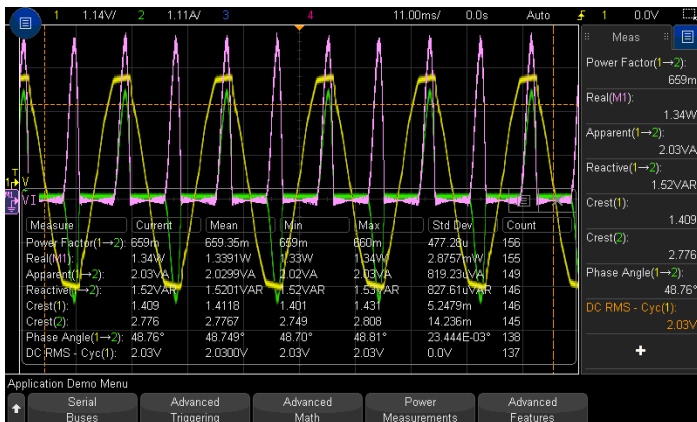
Figure 29: Integrated power measurements make quick work of analyzing power producing and power consuming devices.
